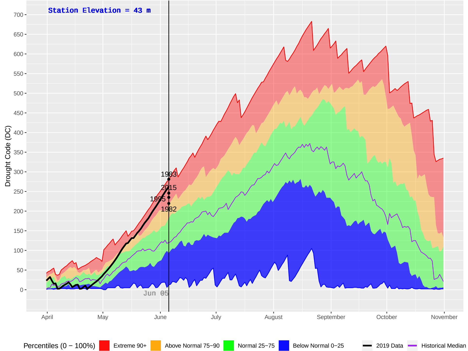
TOBA CAMP (75) : Historical (1970–2018) and Current (2019) Daily Drought Code (DC)
