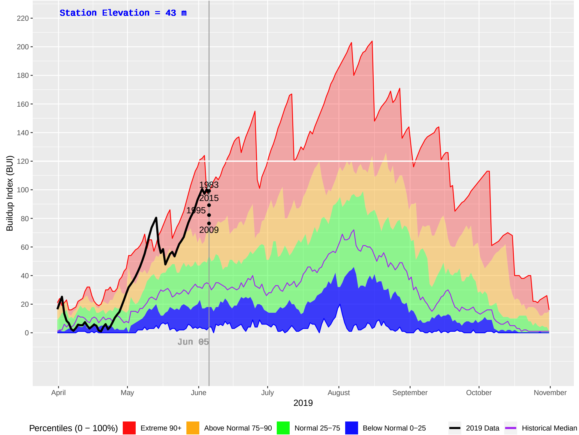
TOBA CAMP (75) : Historical (1970–2018), Current (2019) Daily Buildup Index (BUI)
