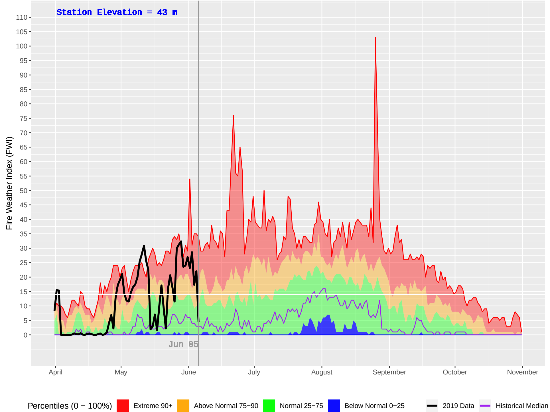
TOBA CAMP (75) : Historical (1970–2018) and Current (2019) Daily Fire Weather Index (FWI)
