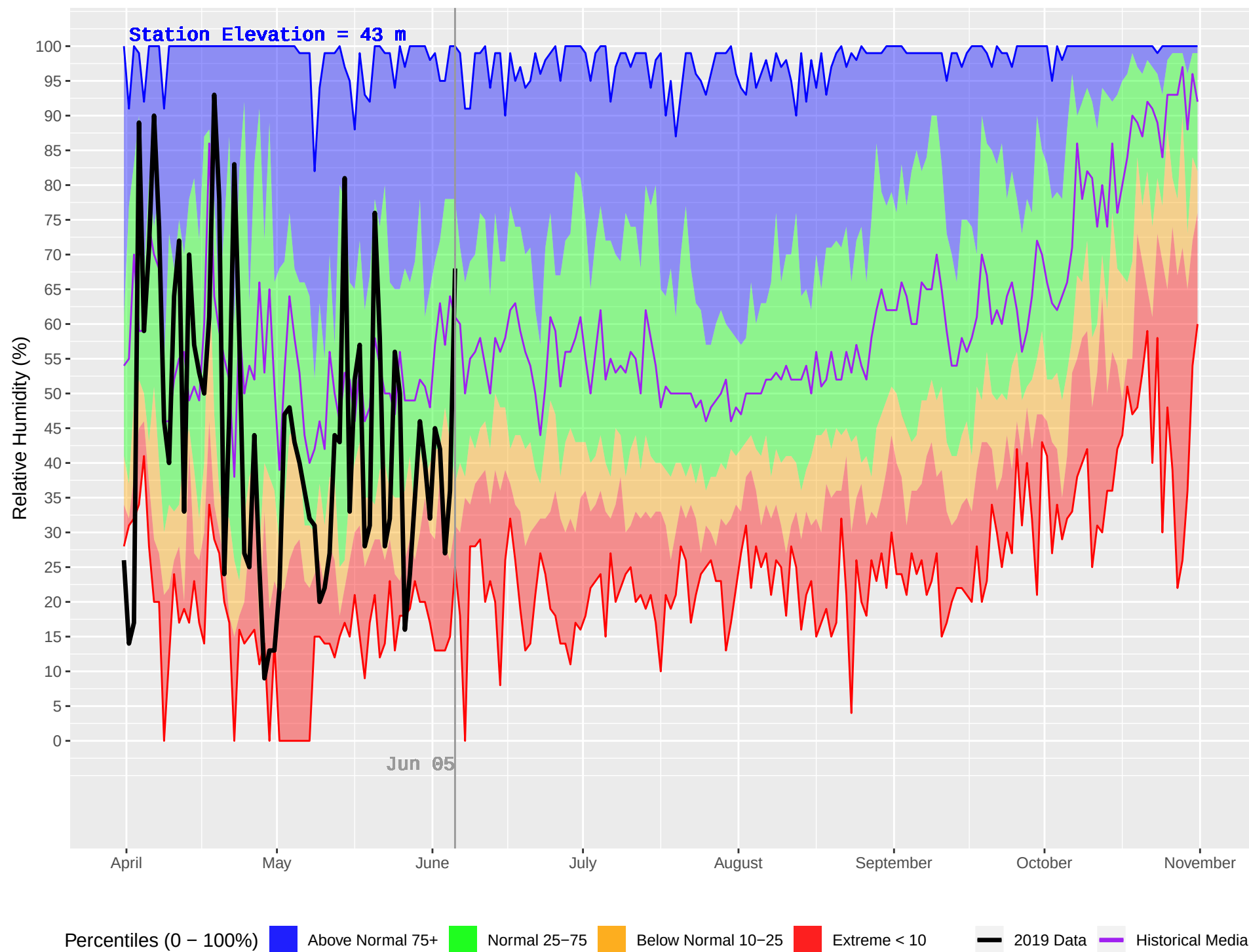
TOBA CAMP (75) : Historical (1970–2018) and Current (2019) Daily Relative Humidity
