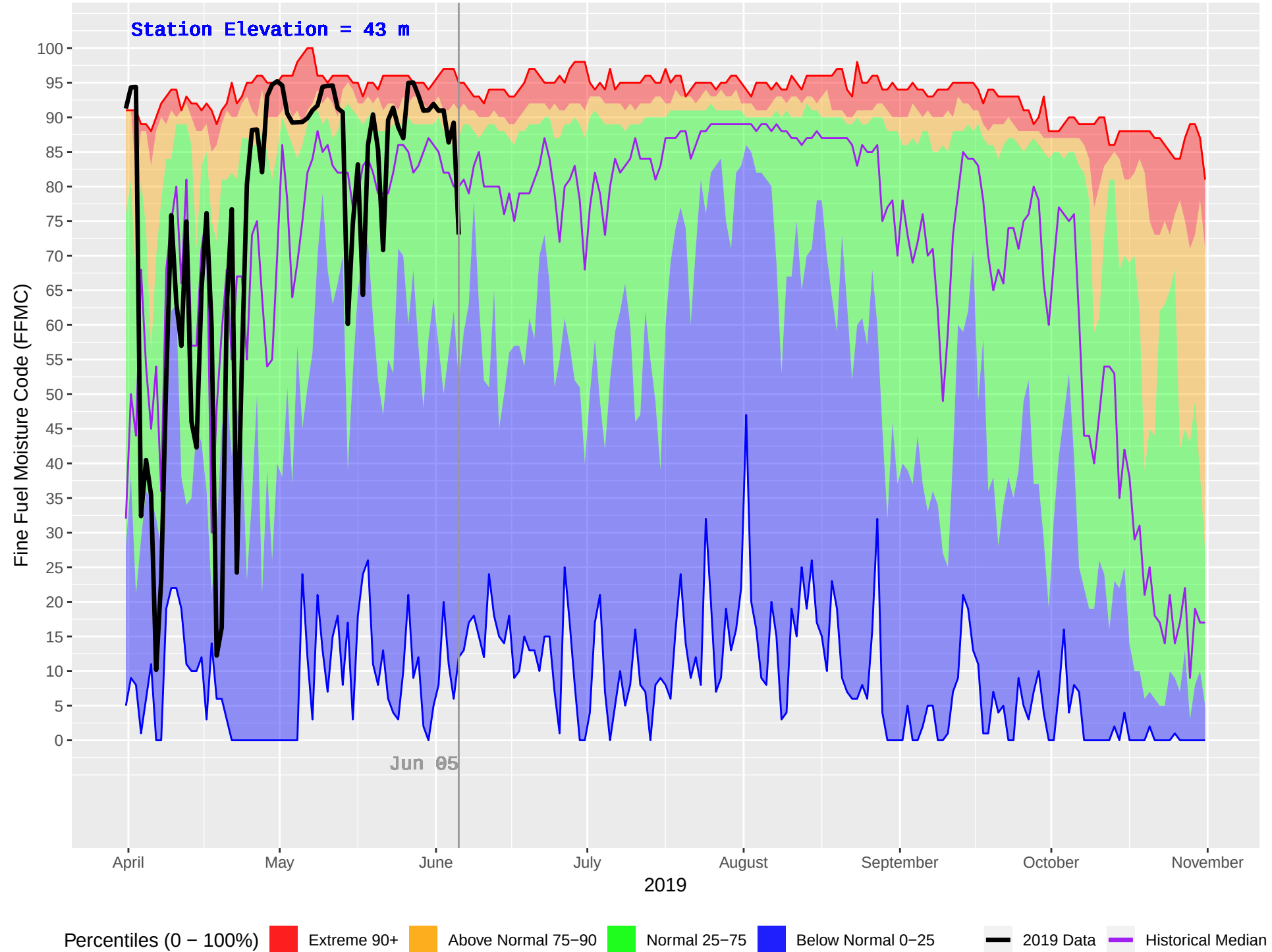
TOBA CAMP (75) : Historical (1970–2018) and Current (2019) Daily Fine Fuel Moisture Code (FFMC)
