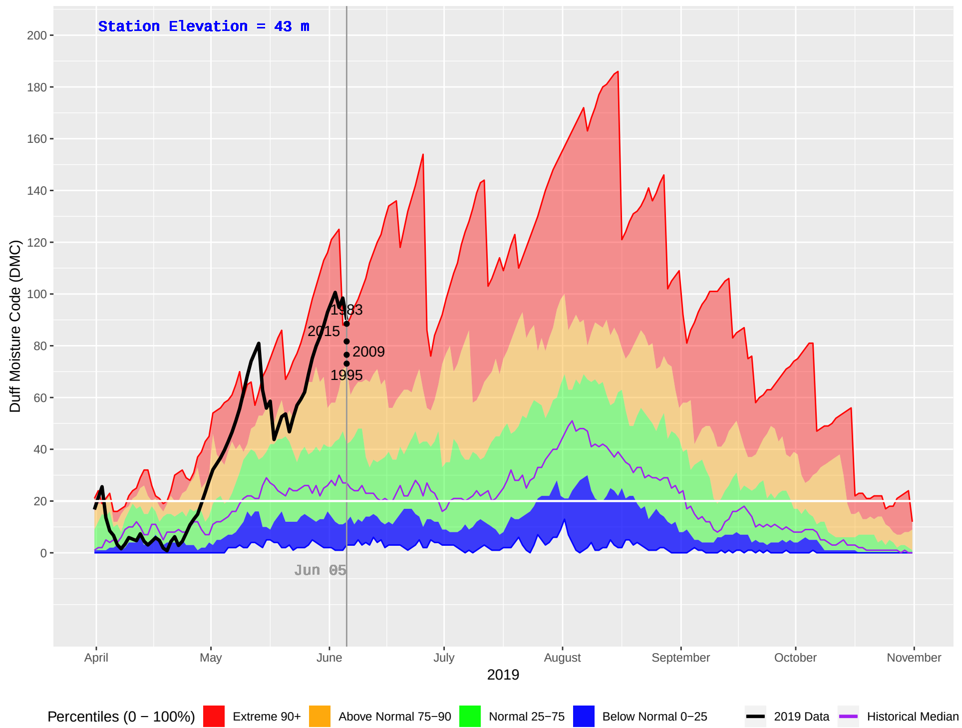
TOBA CAMP (75) : Historical (1970–2018), Current (2019) Daily Duff Moisture Code (DMC)
