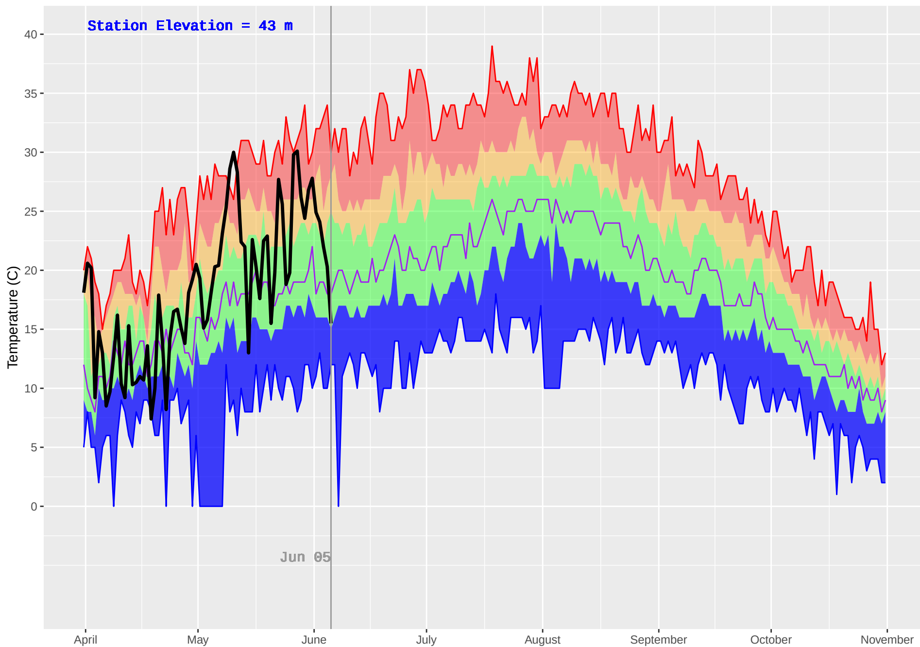
TOBA CAMP (75) : Historical (1970–2018) and Current (2019) Daily Temperature
