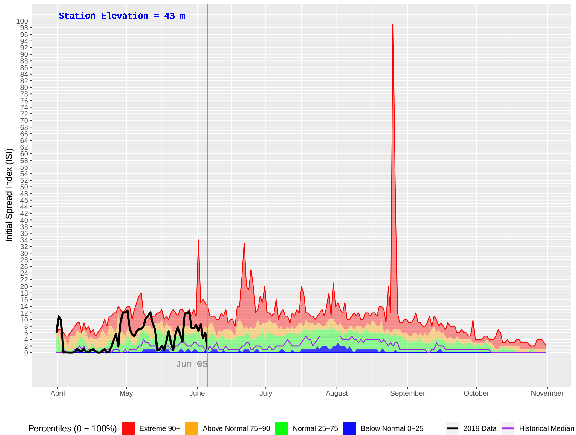
TOBA CAMP (75) : Historical (1970–2018) and Current (2019) Daily Initial Spread Index (ISI)
